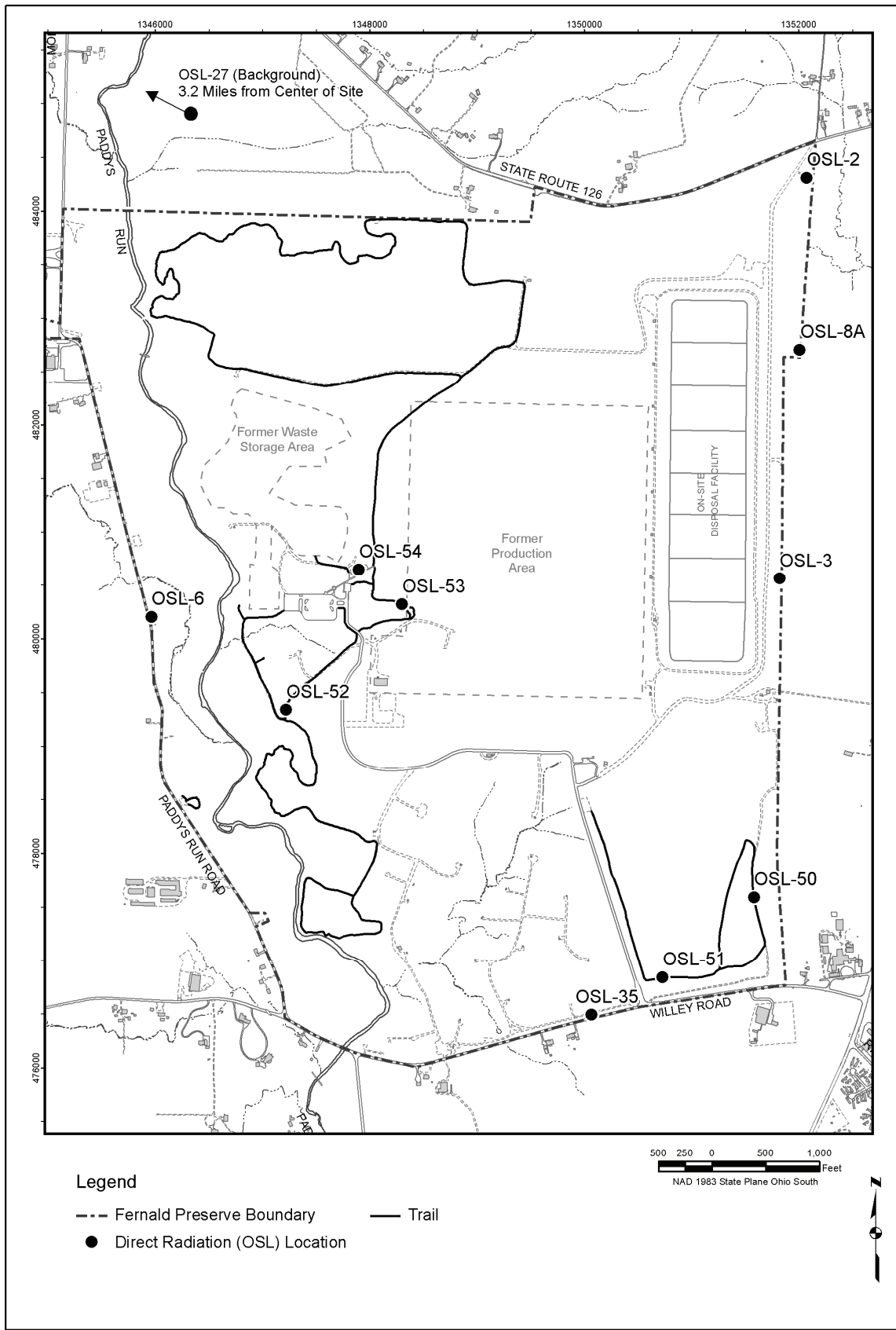
Figure C.1-1. Direct Radiation (OSL) Monitoring Locations
