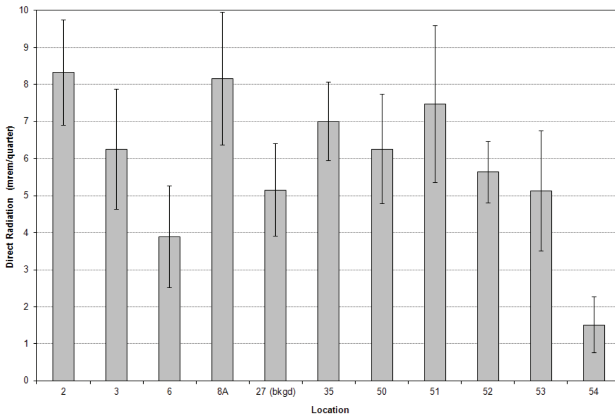
Figure C.1-2. 2011 Mean and 95 Percent Confidence Interval for Quarterly Dosimeter Measurements
